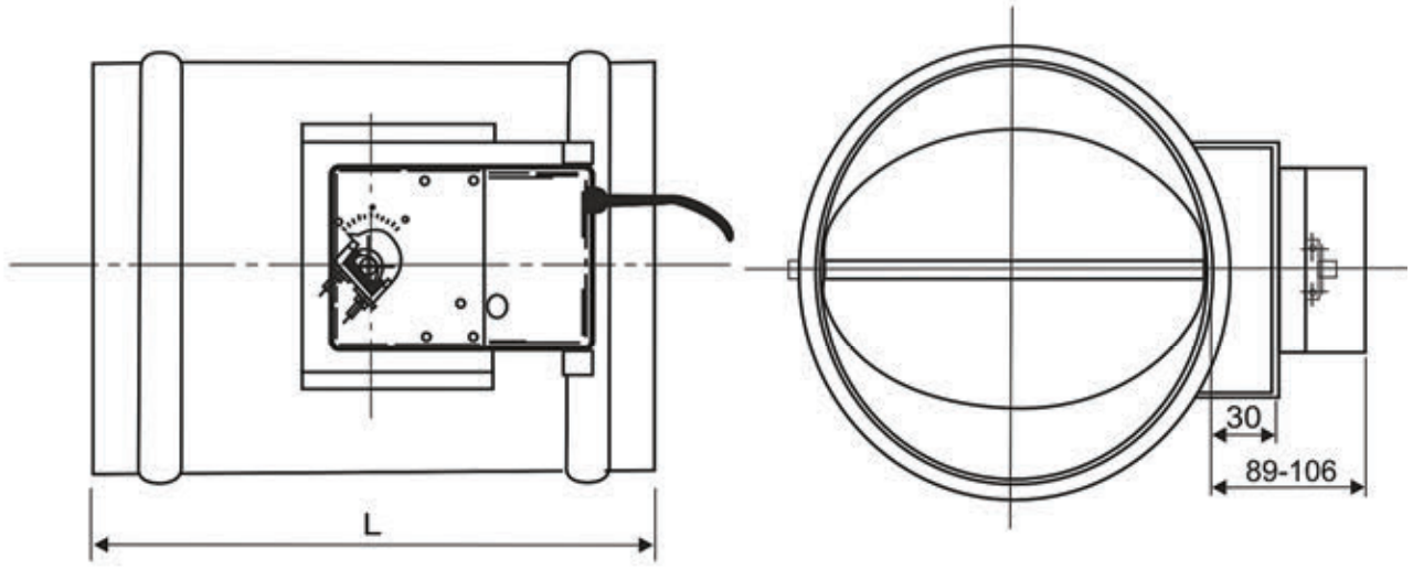
Servomotorlu uygulama / Alternative with actuator
