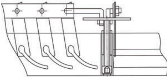
Elle kumandalı With manual control
